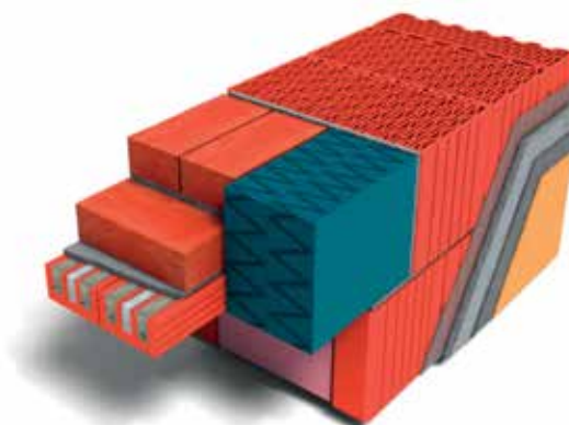
Porotherm A-12 Porotherm Thermo
